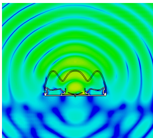
Mainstream patch array sector
