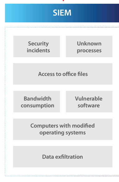
SIEM dashboard
